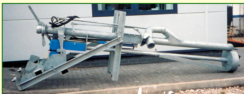
Primex Powerflo variable depth pump, 8-10ft.
